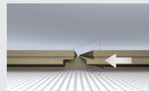
HORIZONTAL INSERTION
